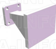
LB-51-15-ASPO Standard Gain Horn Antenna 15-22GHz 15dB Gain Rectangular Waveguide Interface
